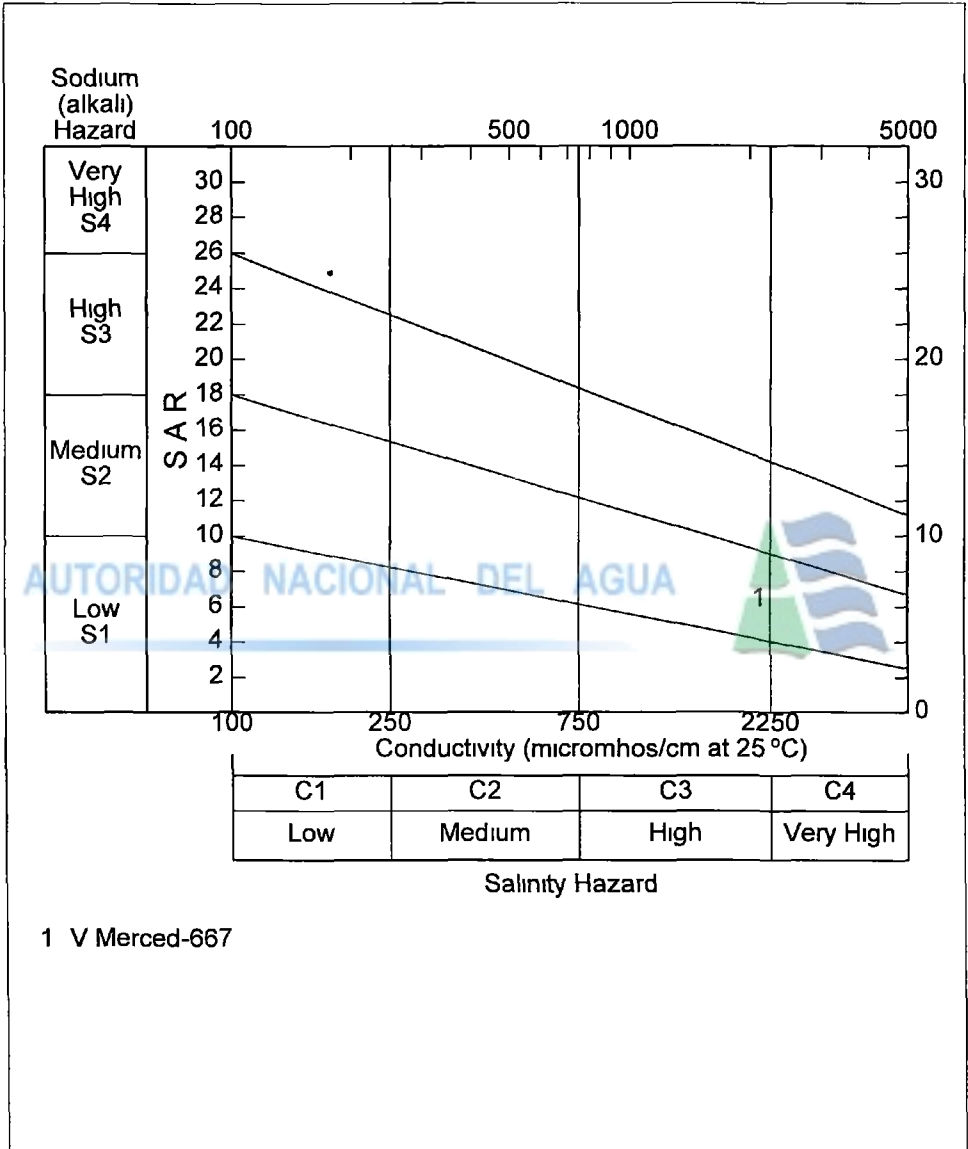
Wilcox Diagram
