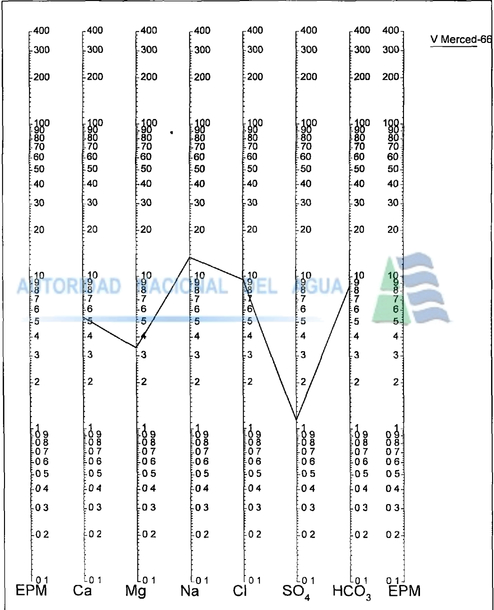
Schoeller Diagram
