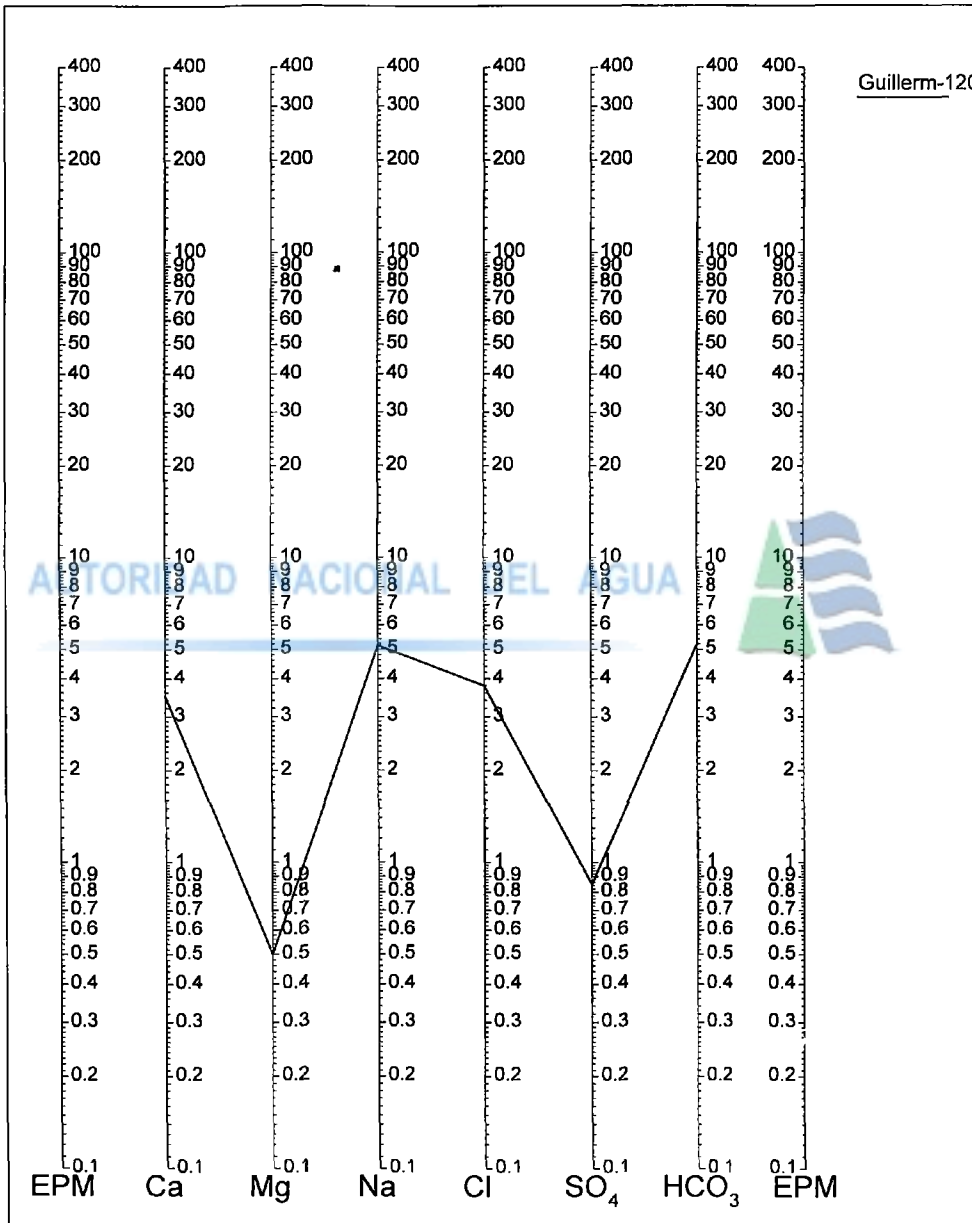
Schoeller Diagram
