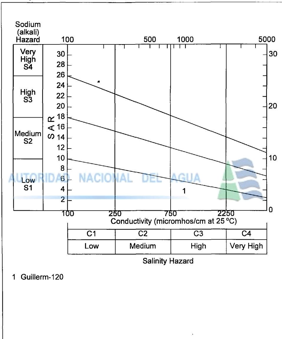
Wilcox Diagram
