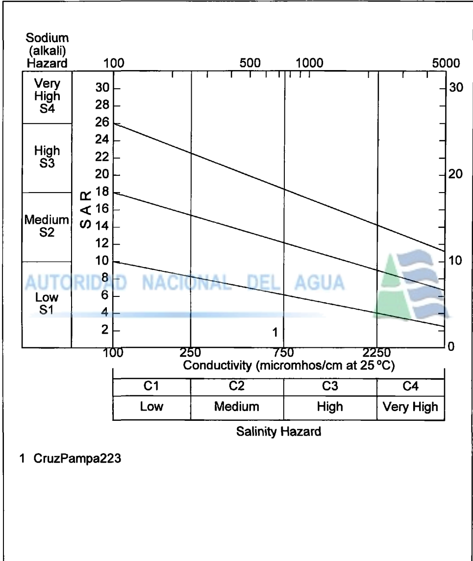
Wilcox Diagram
